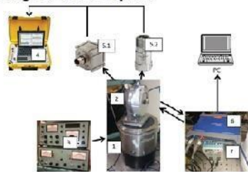
Research of Dynamics of the Precision Mechatronical Line Scale Gage Calibration System
